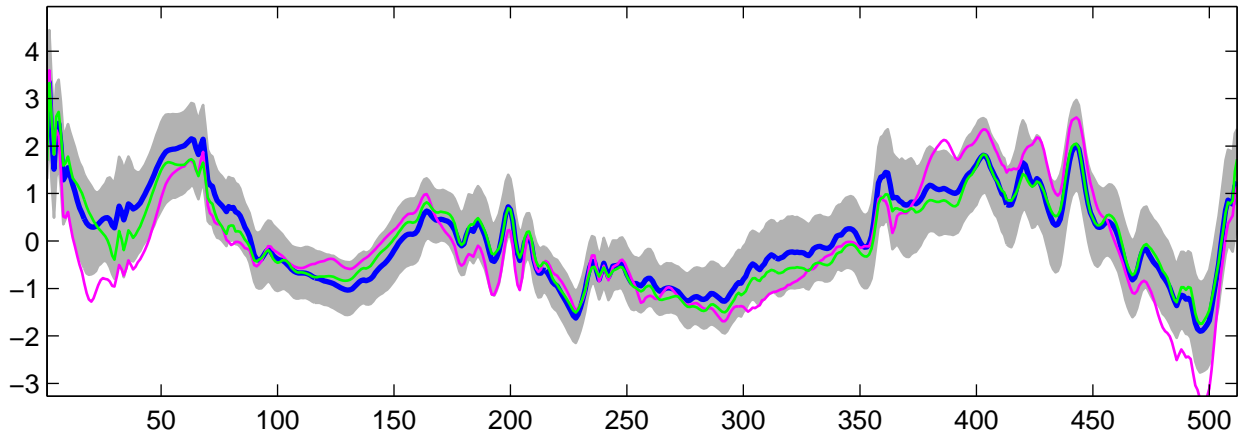
Estimated U_{23}(t) using G-WFMM: DE data, run 8
