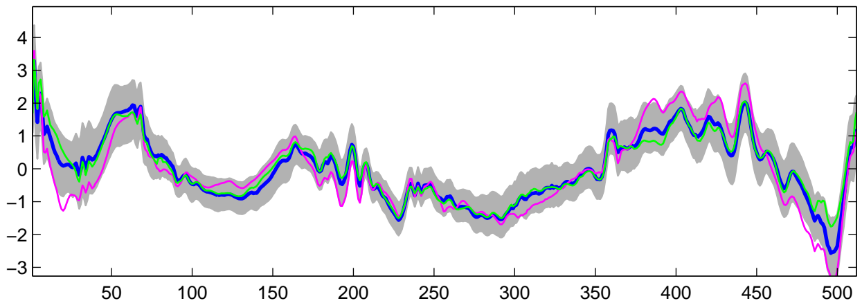
Estimated U_{23}(t) using R-WFMM: DE data, run 8
