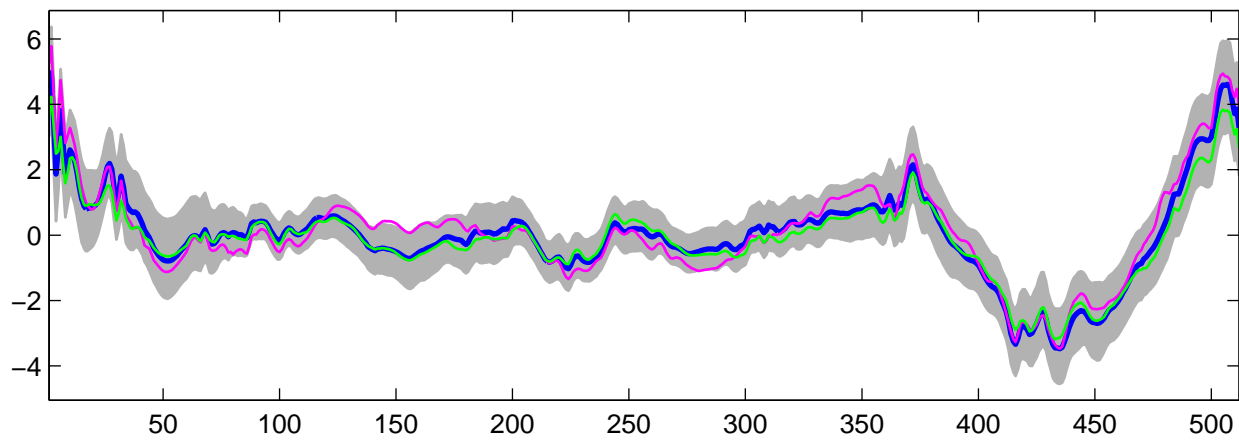
Estimated U_{23}(t) using G-WFMM: Normal data, run 8
