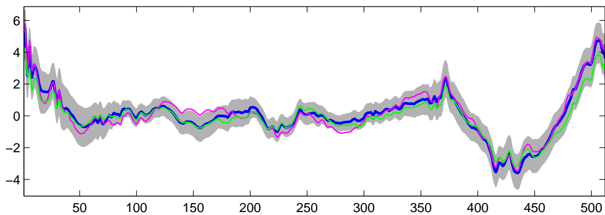
Estimated U_{23}(t) using R-WFMM: Normal data, run 8
