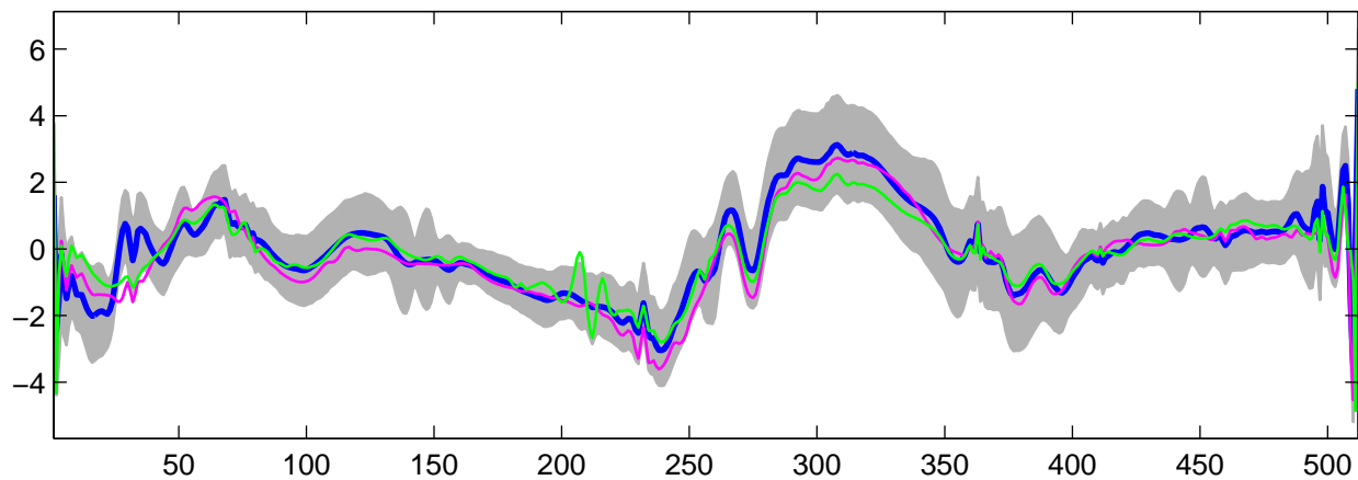
Estimated U_{23}(t) using G-WFMM: t_1 data, run 8
