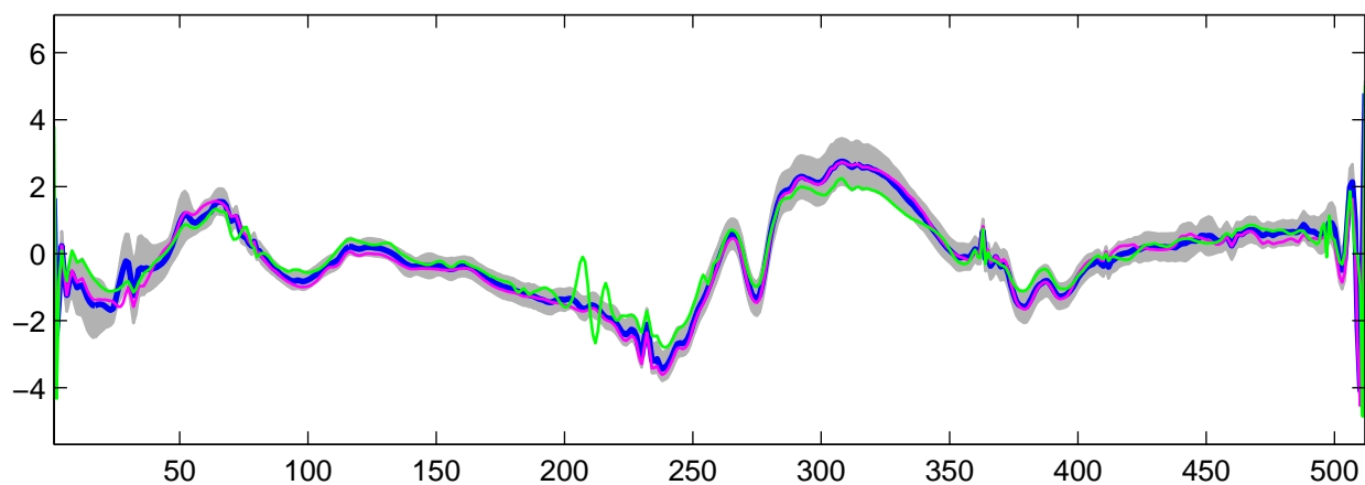
Estimated U_{23}(t) using R-WFMM: t_1 data, run 8
