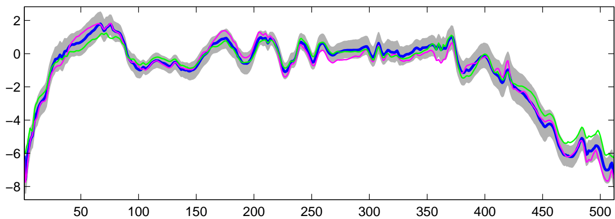
Estimated U_{23}(t) using R-WFMM: t_3 data, run 8
