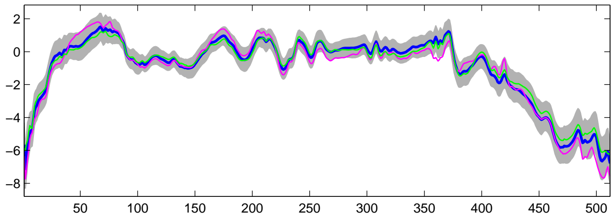
Estimated U_{23}(t) using G-WFMM: t_3 data, run 8
