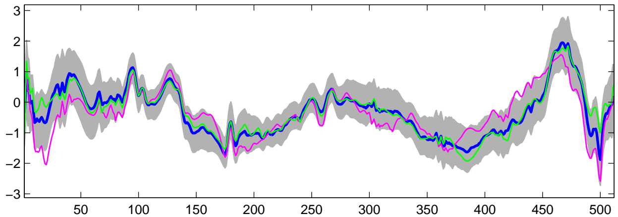
Estimated U_{24}(t) using R-WFMM: DE data, run 8
