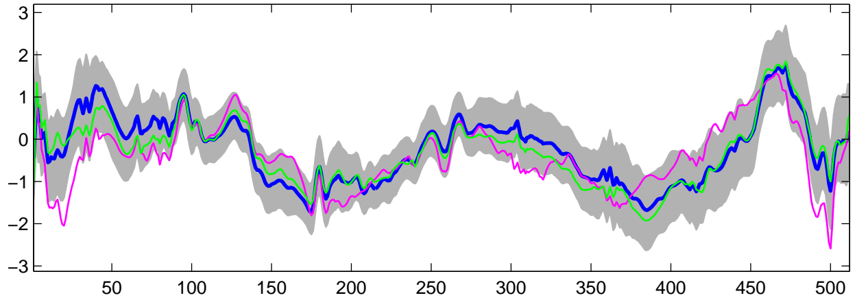
Estimated U_{24}(t) using G-WFMM: DE data, run 8
