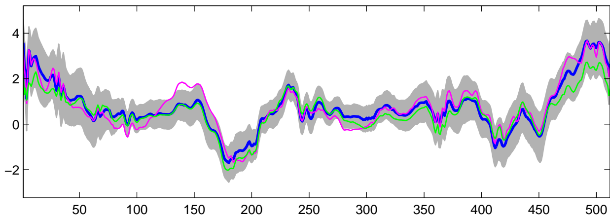
Estimated U_{24}(t) using R-WFMM: Normal data, run 8
