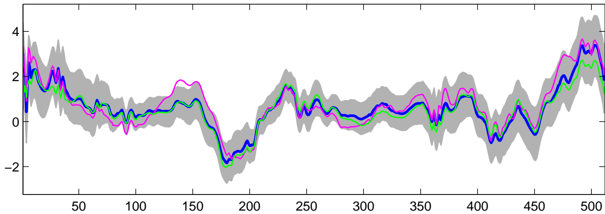
Estimated U_{24}(t) using G-WFMM: Normal data, run 8
