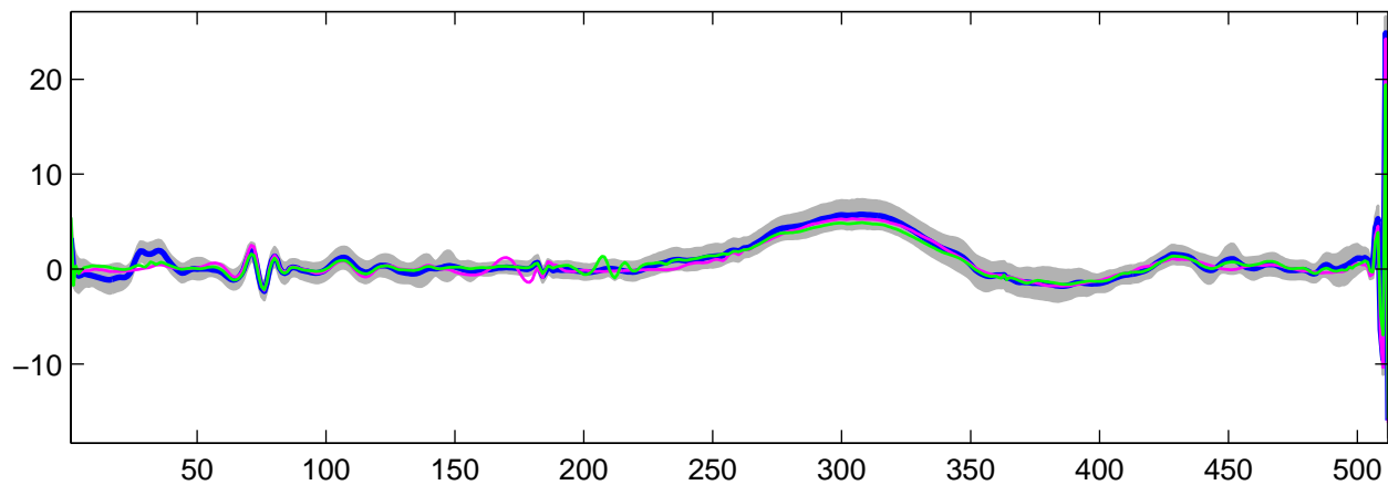
Estimated U_{24}(t) using G-WFMM: t_1 data, run 8
