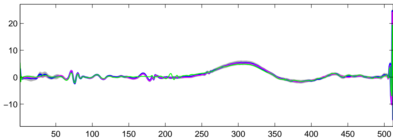
Estimated U_{24}(t) using R-WFMM: t_1 data, run 8
