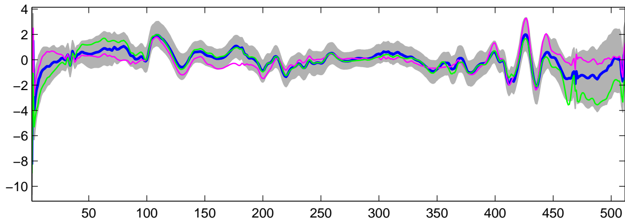
Estimated U_{24}(t) using G-WFMM: t_2 data, run 8
