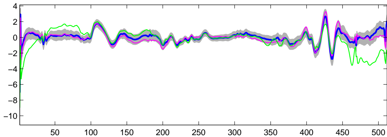
Estimated U_{24}(t) using R-WFMM: t_2 data, run 8
