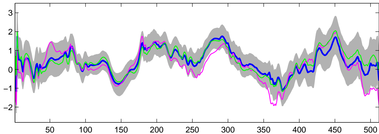
Estimated U_{24}(t) using G-WFMM: t_3 data, run 8
