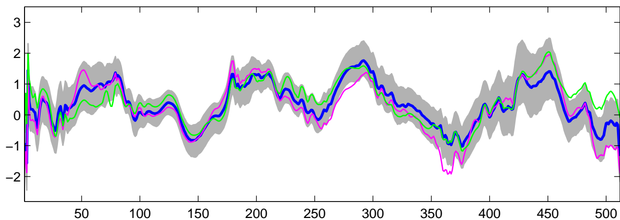
Estimated U_{24}(t) using R-WFMM: t_3 data, run 8
