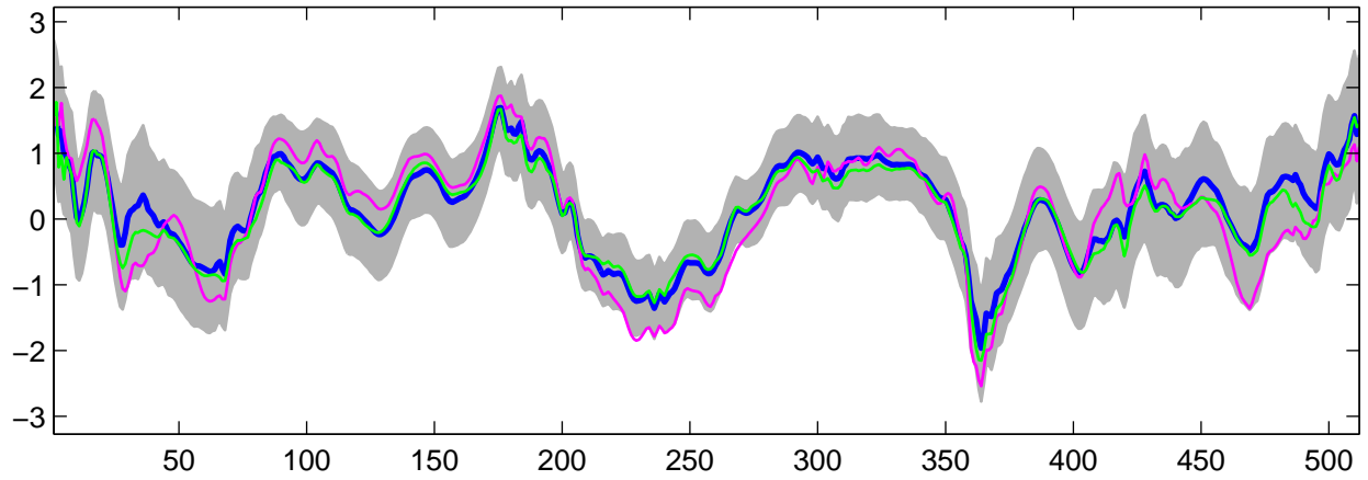
Estimated U_{25}(t) using G-WFMM: DE data, run 8
