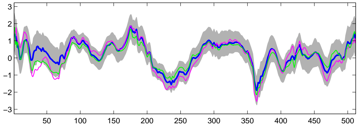
Estimated U_{25}(t) using R-WFMM: DE data, run 8
