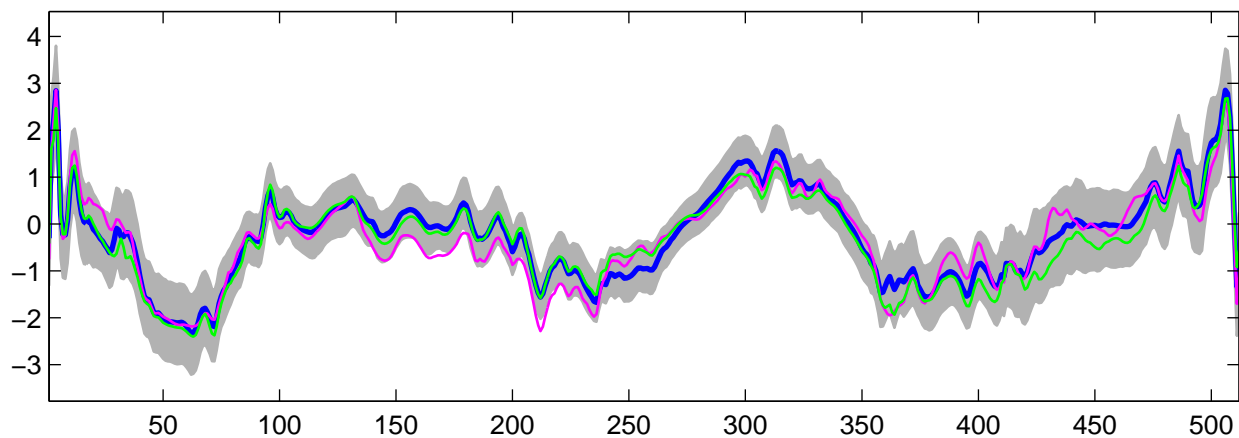
Estimated U_{25}(t) using R-WFMM: Normal data, run 8
