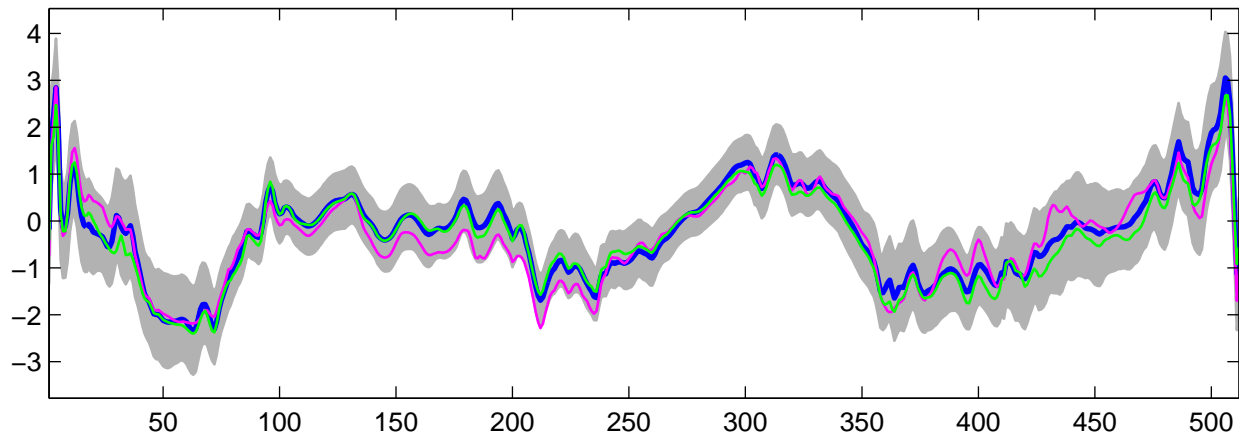
Estimated U_{25}(t) using G-WFMM: Normal data, run 8
