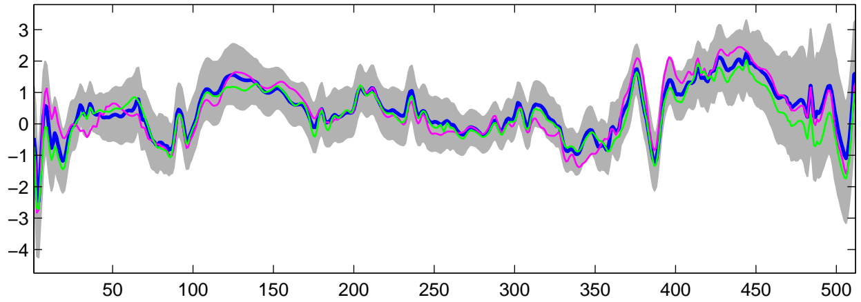
Estimated U_{25}(t) using G-WFMM: t_2 data, run 8
