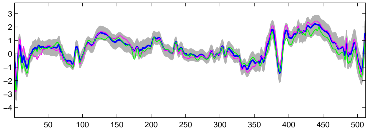
Estimated U_{25}(t) using R-WFMM: t_2 data, run 8
