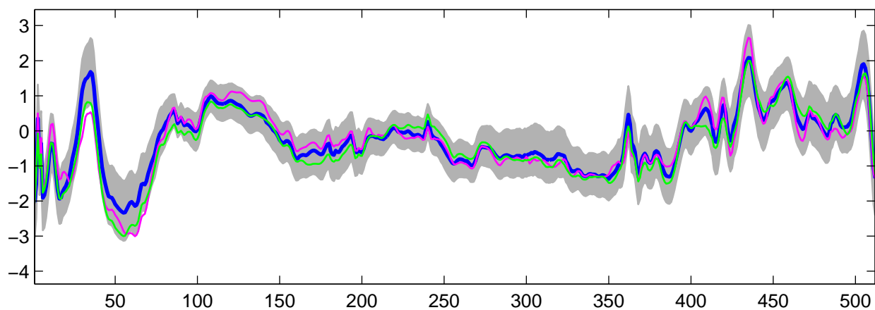
Estimated U_{26}(t) using R-WFMM: DE data, run 8
