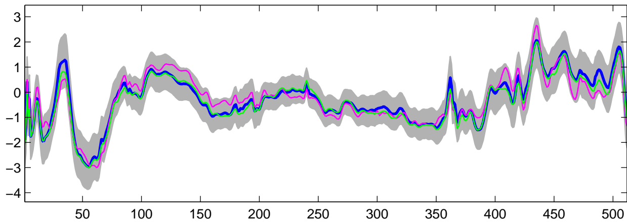
Estimated U_{26}(t) using G-WFMM: DE data, run 8
