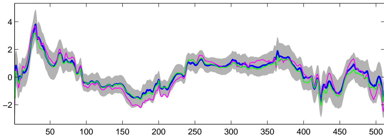
Estimated U_{26}(t) using G-WFMM: Normal data, run 8
