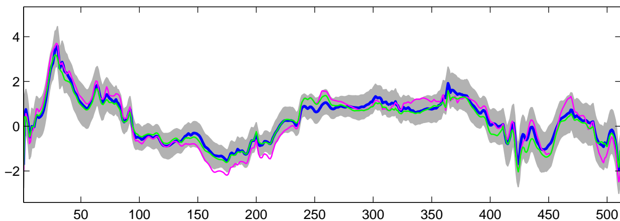
Estimated U_{26}(t) using R-WFMM: Normal data, run 8
