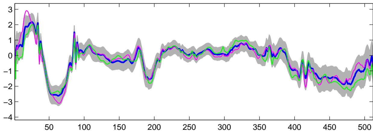
Estimated U_{26}(t) using R-WFMM: t_2 data, run 8
