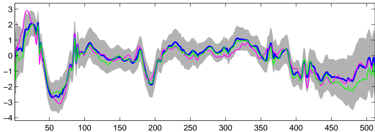
Estimated U_{26}(t) using G-WFMM: t_2 data, run 8
