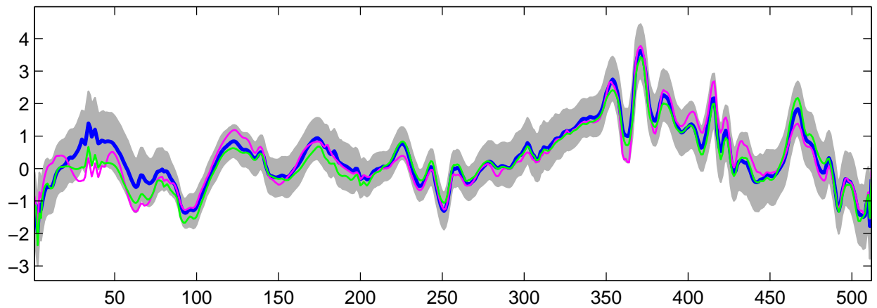
Estimated U_{27}(t) using R-WFMM: DE data, run 8
