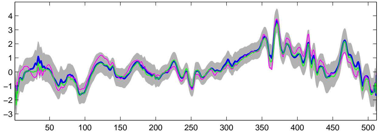
Estimated U_{27}(t) using G-WFMM: DE data, run 8
