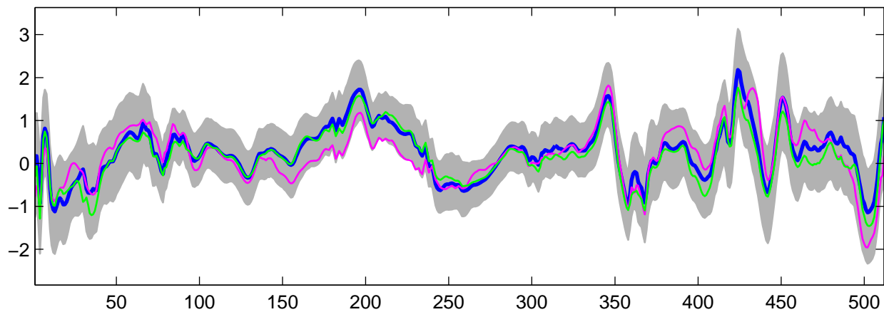
Estimated U_{27}(t) using G-WFMM: Normal data, run 8
