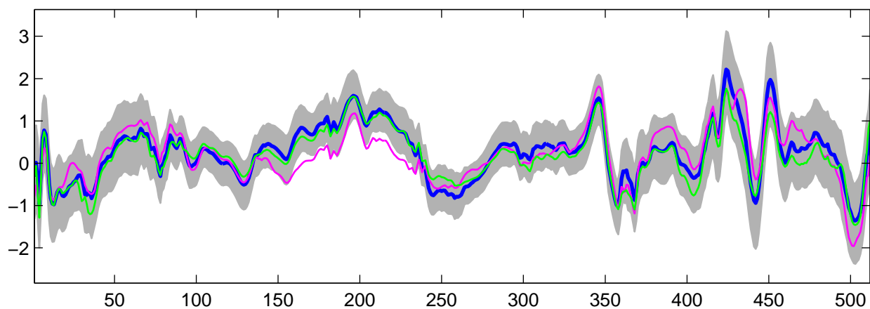
Estimated U_{27}(t) using R-WFMM: Normal data, run 8
