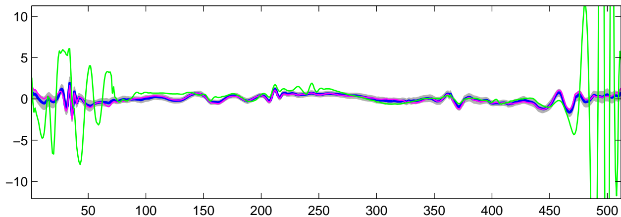
Estimated U_{27}(t) using R-WFMM: t_1 data, run 8
