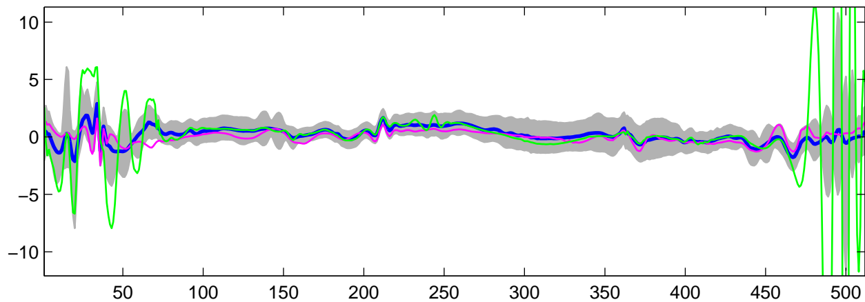
Estimated U_{27}(t) using G-WFMM: t_1 data, run 8
