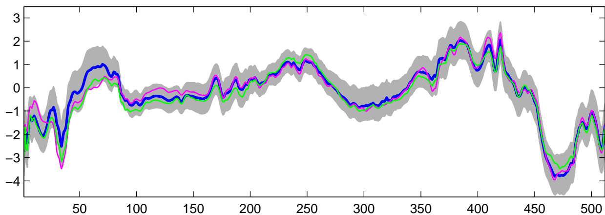
Estimated U_{28}(t) using R-WFMM: DE data, run 8
