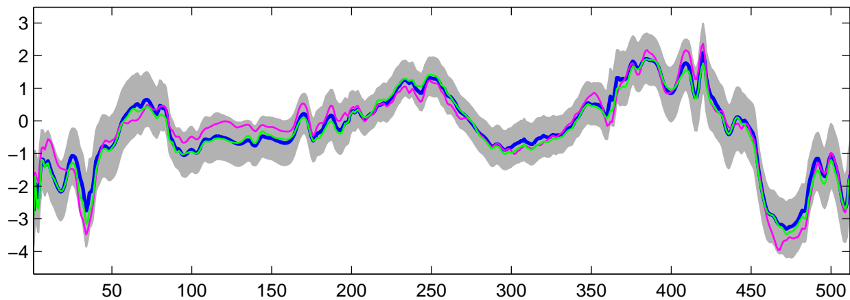
Estimated U_{28}(t) using G-WFMM: DE data, run 8
