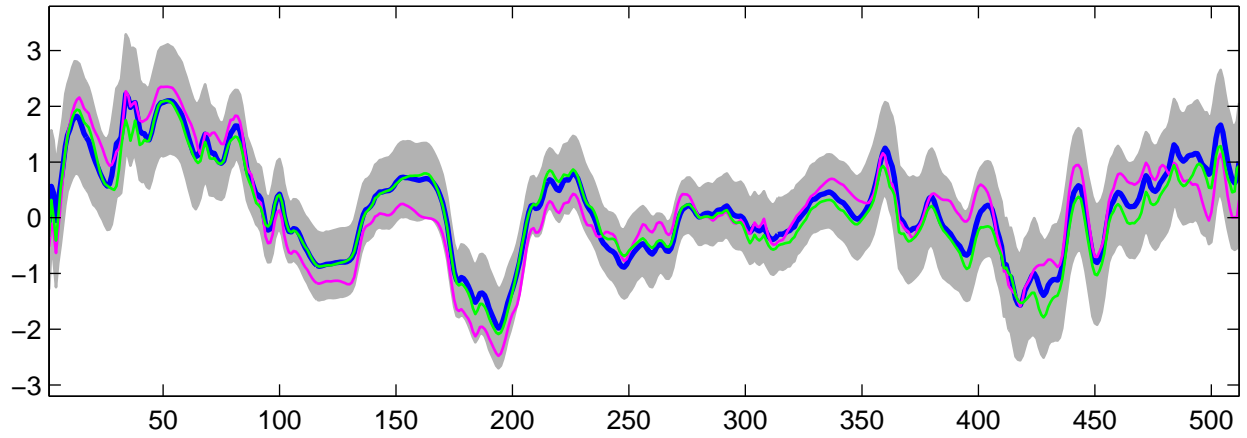
Estimated U_{28}(t) using G-WFMM: Normal data, run 8
