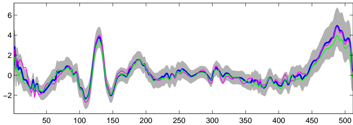
Estimated U_{28}(t) using G-WFMM: t_2 data, run 8
