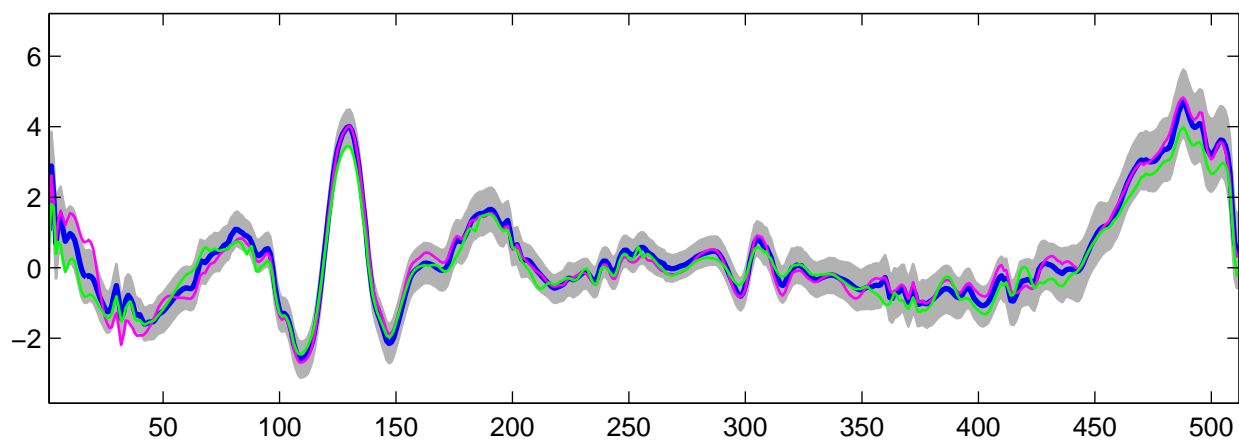
Estimated U_{28}(t) using R-WFMM: t_2 data, run 8
