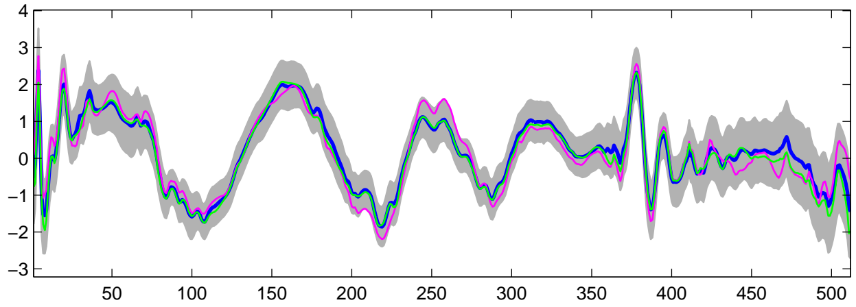
Estimated U_{28}(t) using G-WFMM: t_3 data, run 8
