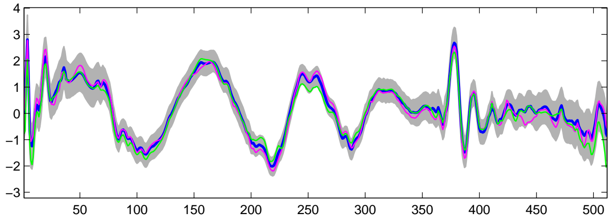
Estimated U_{28}(t) using R-WFMM: t_3 data, run 8
