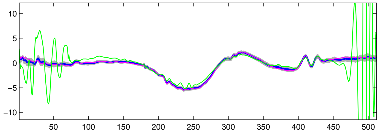
Estimated U_{29}(t) using R-WFMM: t_1 data, run 8
