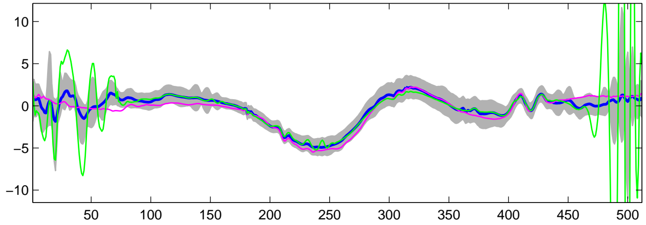
Estimated U_{29}(t) using G-WFMM: t_1 data, run 8
