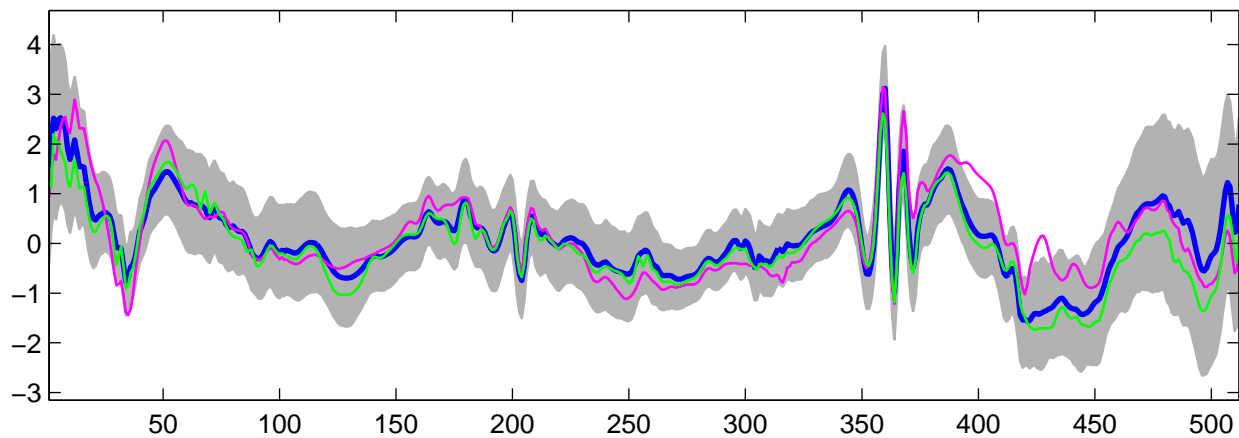
Estimated U_{29}(t) using G-WFMM: t_2 data, run 8
