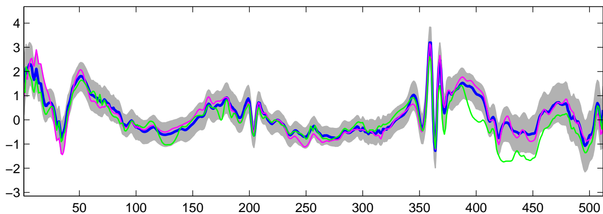
Estimated U_{29}(t) using R-WFMM: t_2 data, run 8
