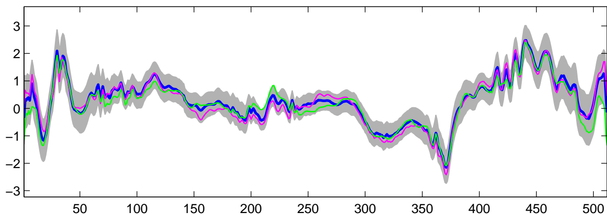
Estimated U_{29}(t) using R-WFMM: t_3 data, run 8
