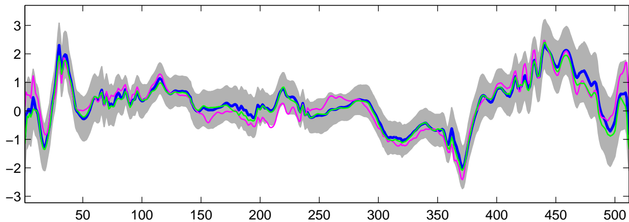
Estimated U_{29}(t) using G-WFMM: t_3 data, run 8
