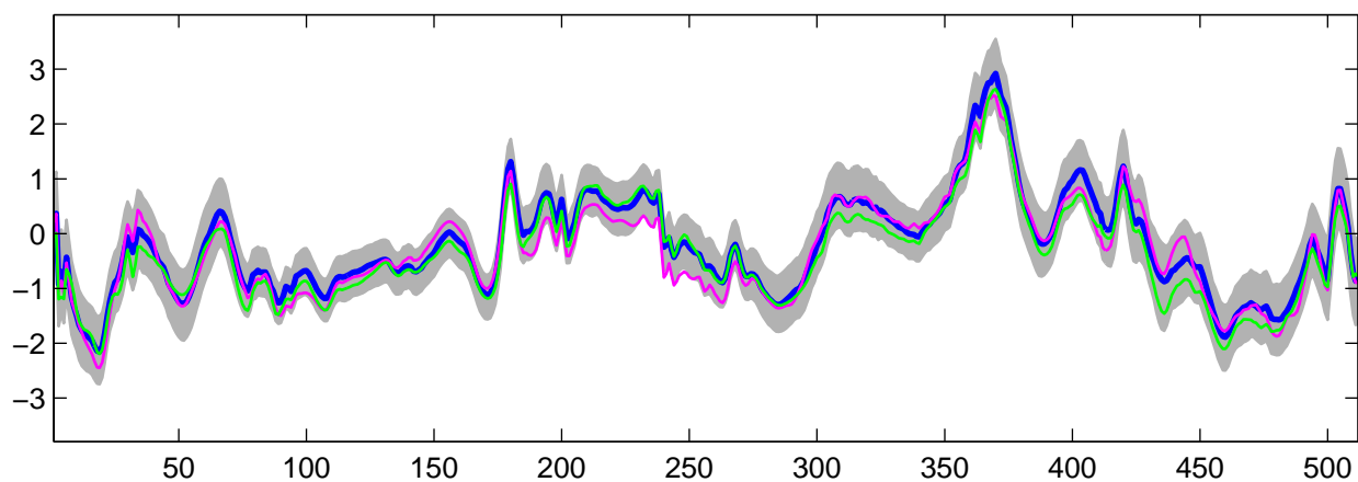
Estimated U_2(t) using R-WFMM: DE data, run 8
