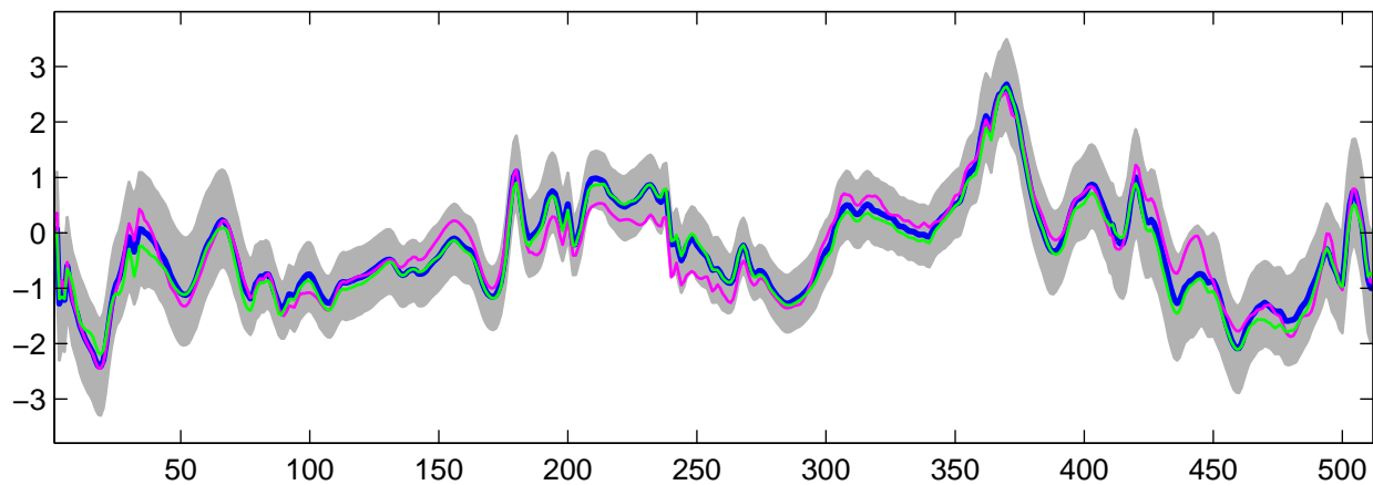
Estimated U_2(t) using G-WFMM: DE data, run 8
