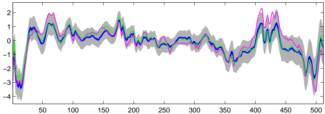
Estimated U_2(t) using R-WFMM: Normal data, run 8
