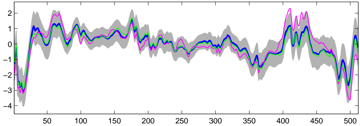
Estimated U_2(t) using G-WFMM: Normal data, run 8
