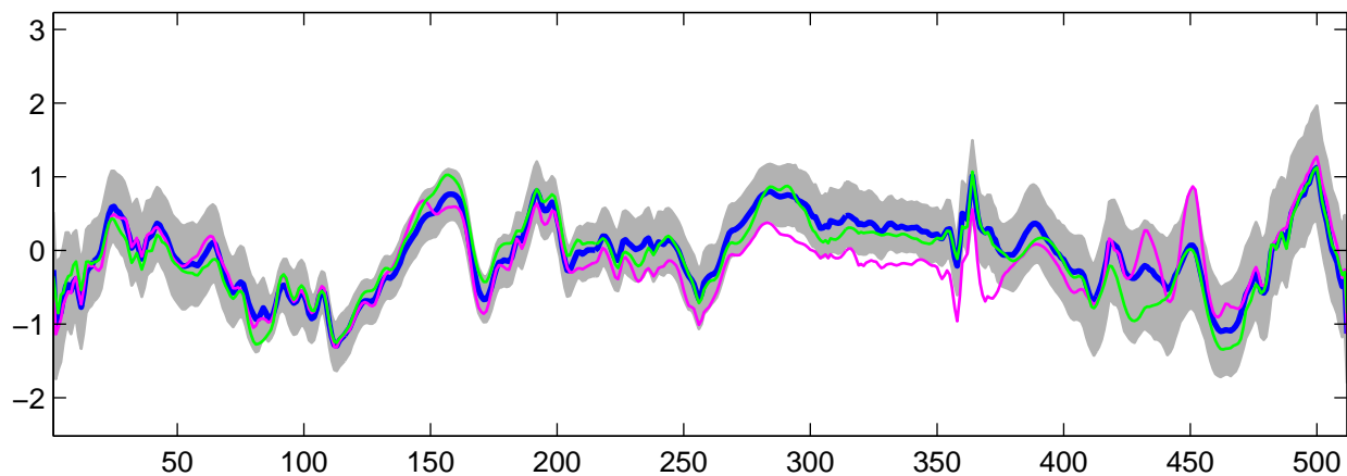
Estimated U_2(t) using R-WFMM: t_3 data, run 8
