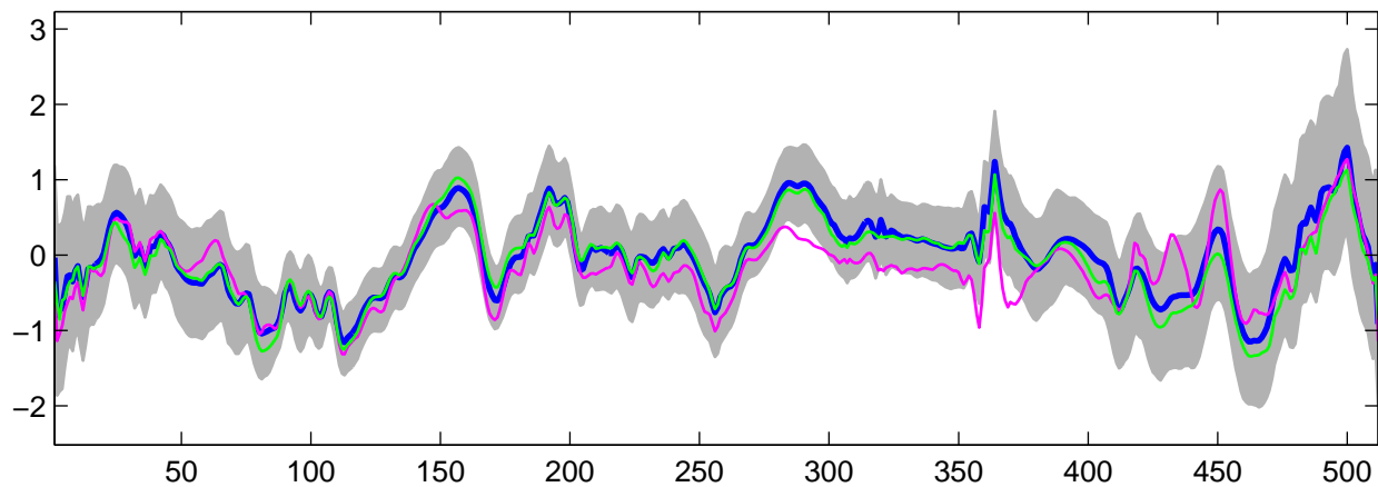
Estimated U_2(t) using G-WFMM: t_3 data, run 8
