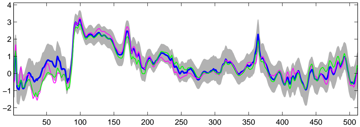
Estimated U_{30}(t) using R-WFMM: DE data, run 8
