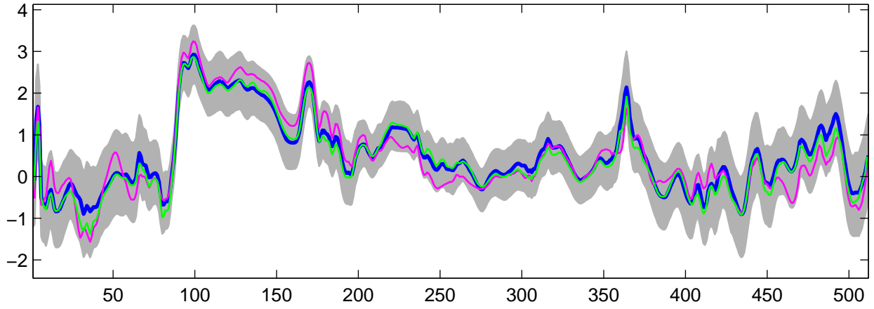
Estimated U_{30}(t) using G-WFMM: DE data, run 8
