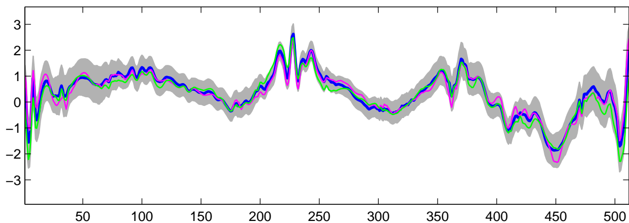
Estimated U_{30}(t) using R-WFMM: t_3 data, run 8
