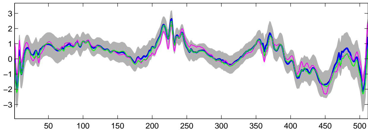
Estimated U_{30}(t) using G-WFMM: t_3 data, run 8
