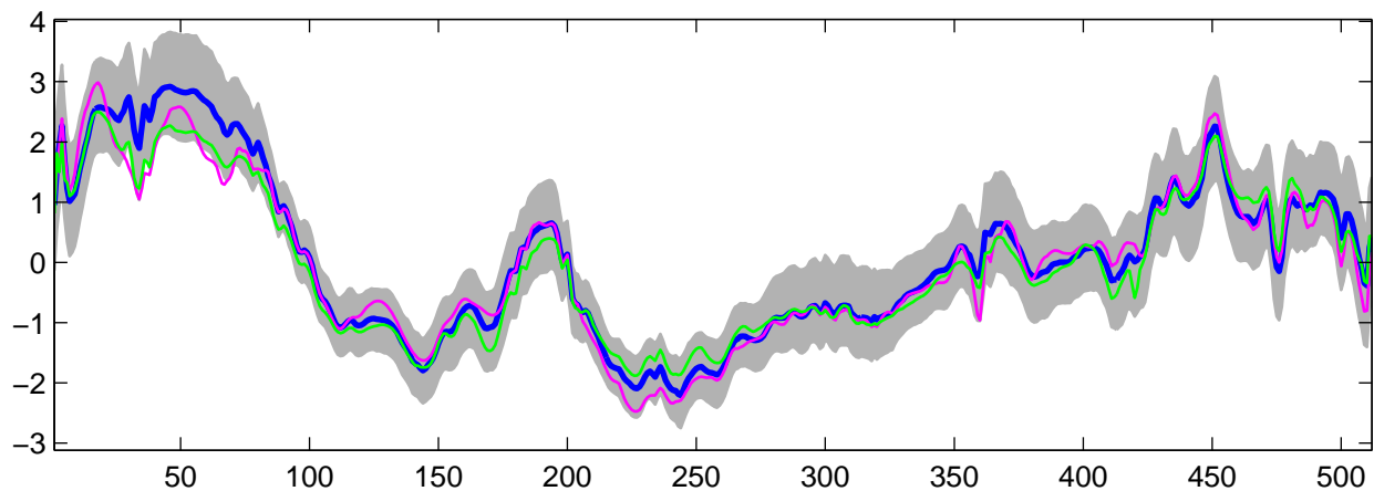
Estimated U_{31}(t) using R-WFMM: DE data, run 8
