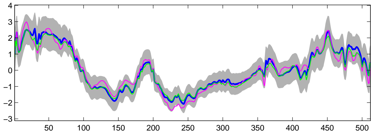
Estimated U_{31}(t) using G-WFMM: DE data, run 8
