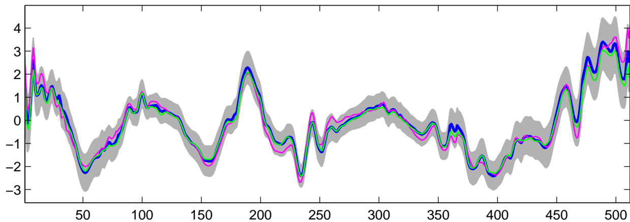
Estimated U_{31}(t) using G-WFMM: t_3 data, run 8
