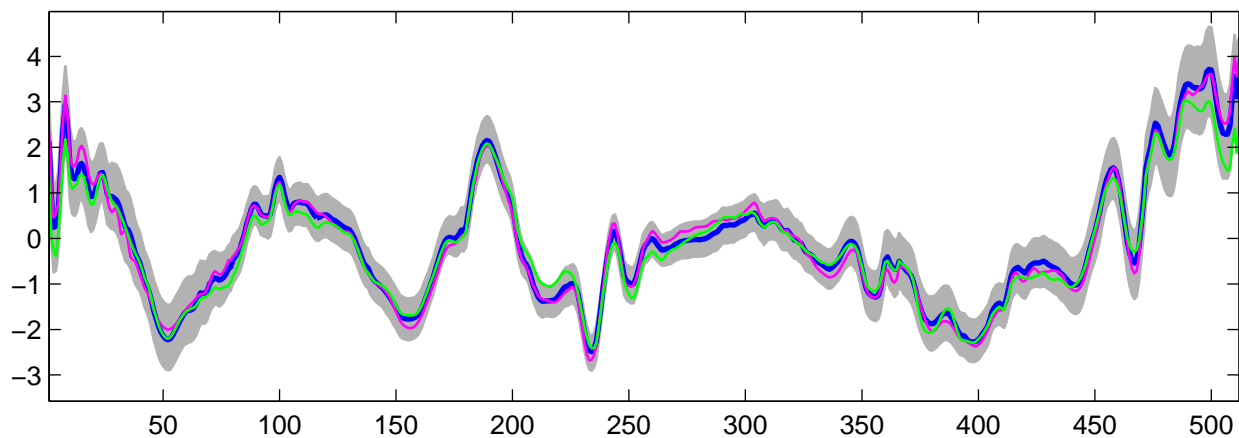
Estimated U_{31}(t) using R-WFMM: t_3 data, run 8
