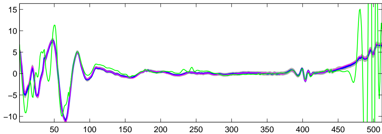
Estimated U_{32}(t) using R-WFMM: t_1 data, run 8
