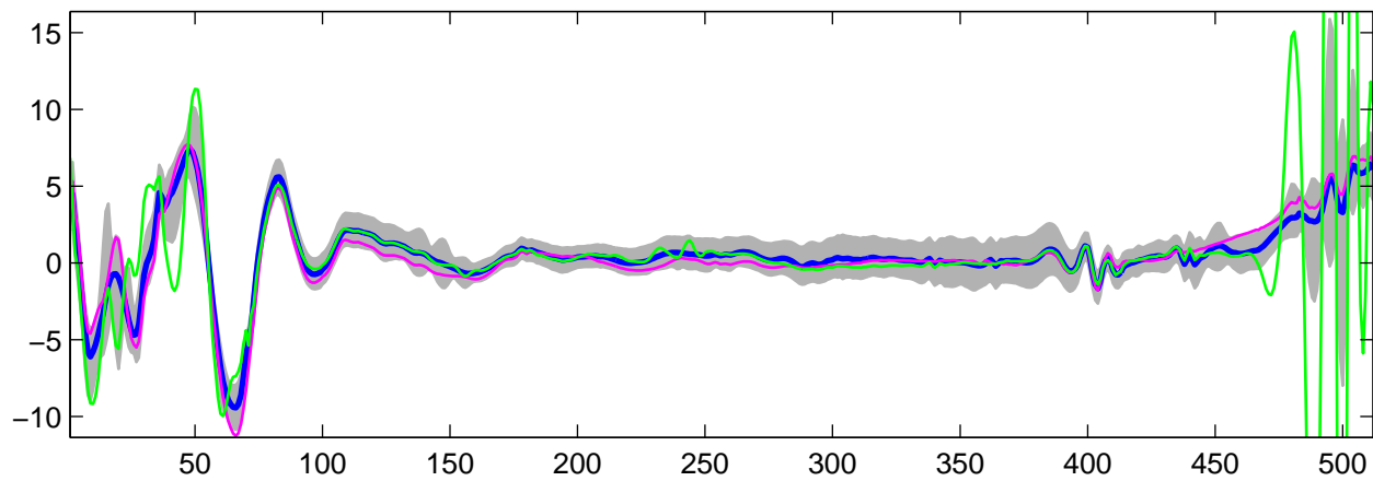
Estimated U_{32}(t) using G-WFMM: t_1 data, run 8
