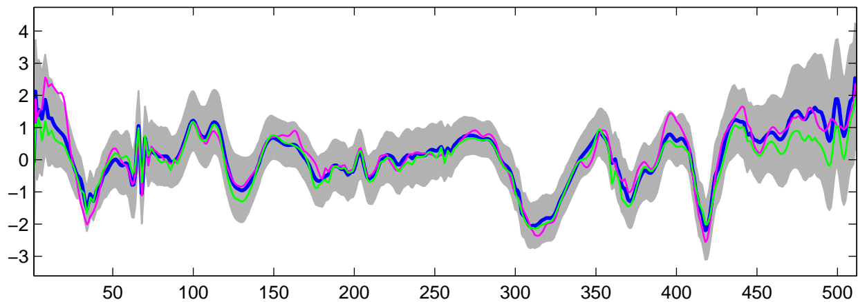
Estimated U_{32}(t) using G-WFMM: t_2 data, run 8
