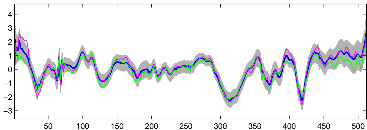
Estimated U_{32}(t) using R-WFMM: t_2 data, run 8
