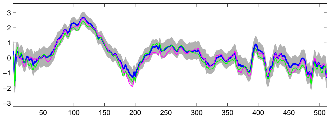
Estimated U_3(t) using R-WFMM: DE data, run 8
