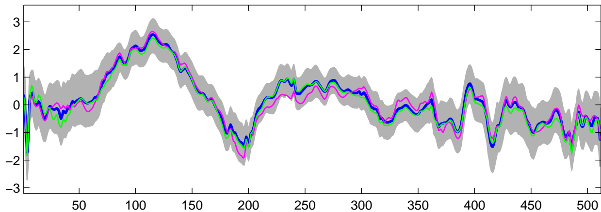
Estimated U_3(t) using G-WFMM: DE data, run 8
