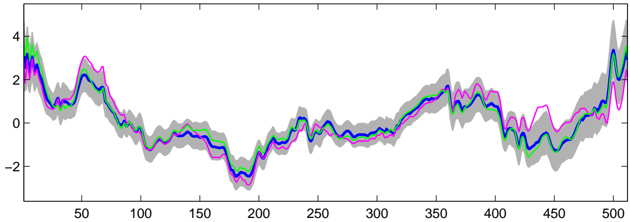
Estimated U_3(t) using R-WFMM: Normal data, run 8
