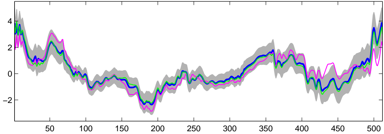
Estimated U_3(t) using G-WFMM: Normal data, run 8
