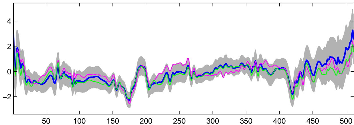
Estimated U_3(t) using G-WFMM: t_2 data, run 8
