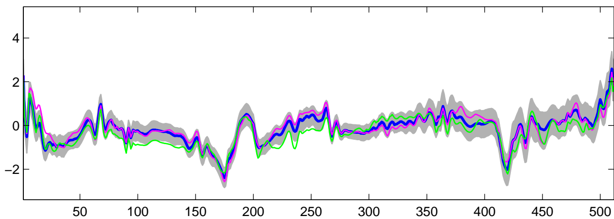
Estimated U_3(t) using R-WFMM: t_2 data, run 8
