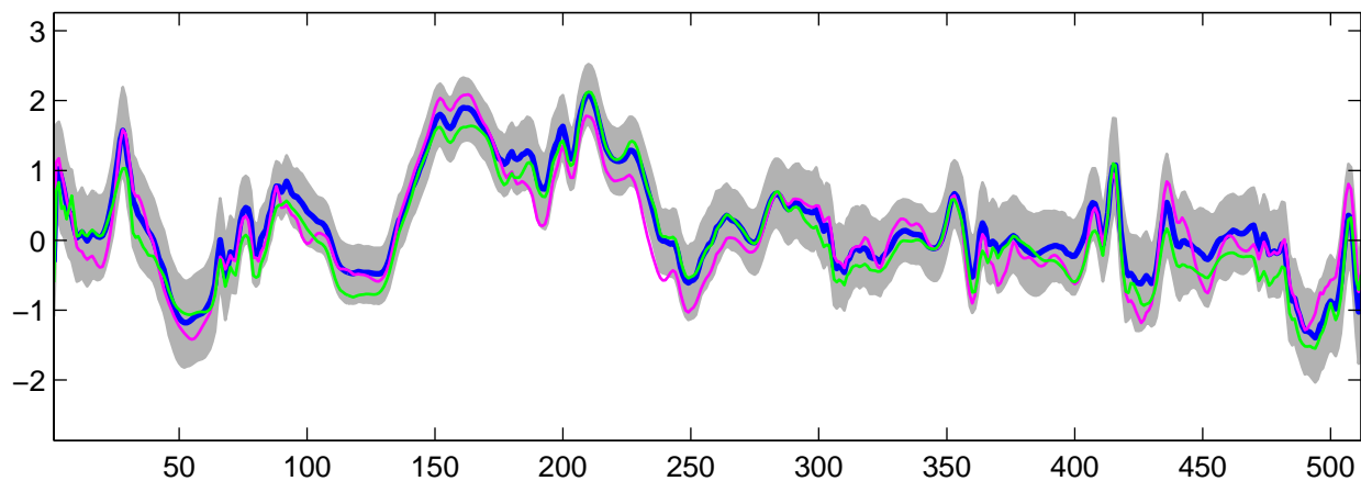
Estimated U_4(t) using R-WFMM: DE data, run 8
