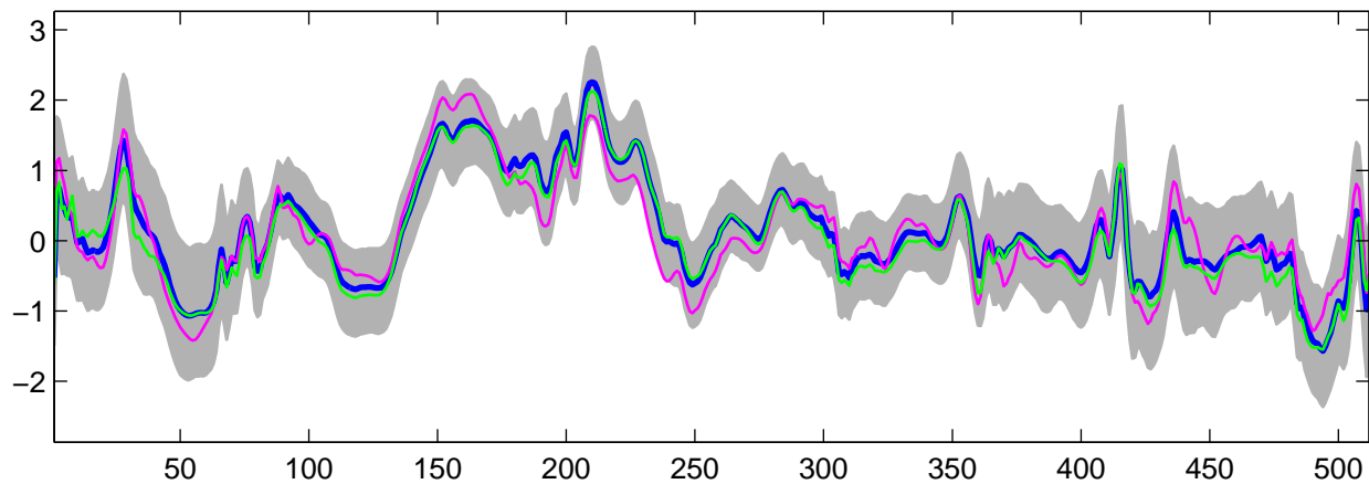
Estimated U_4(t) using G-WFMM: DE data, run 8
