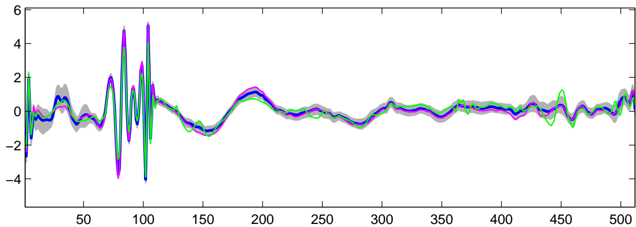
Estimated U_4(t) using R-WFMM: t_1 data, run 8
