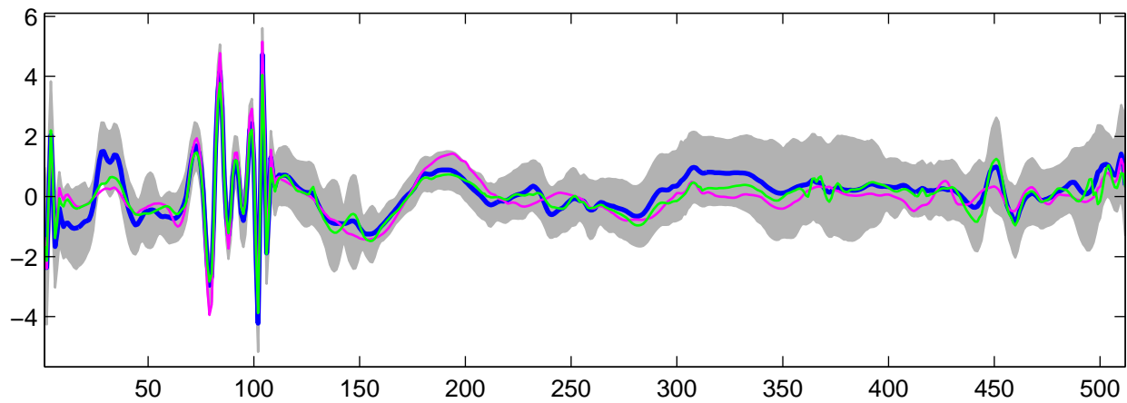
Estimated U_4(t) using G-WFMM: t_1 data, run 8
