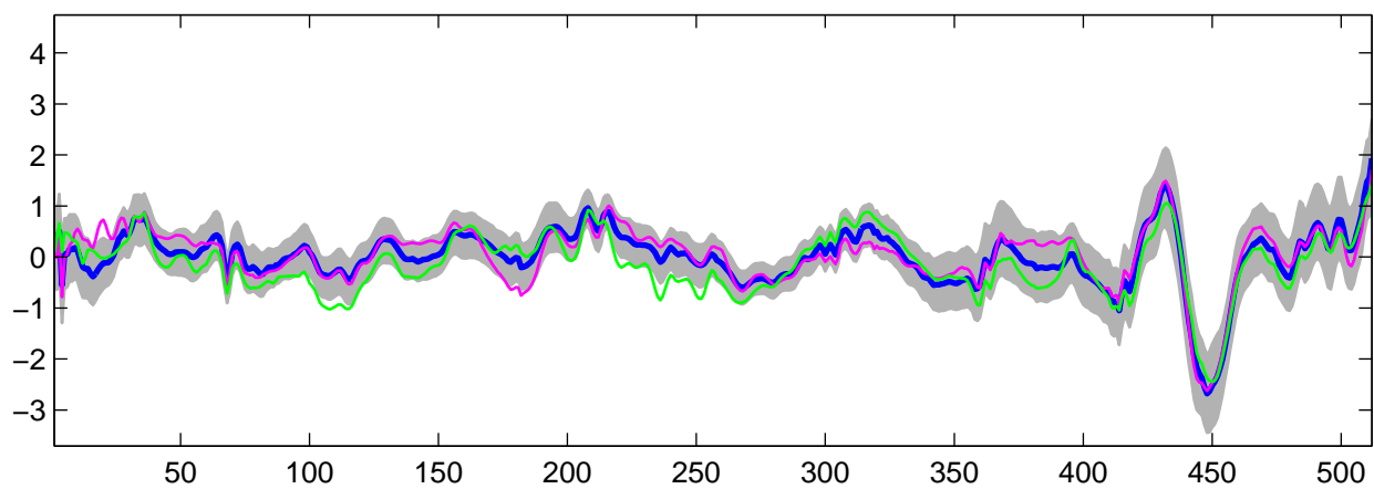
Estimated U_4(t) using R-WFMM: t_2 data, run 8
