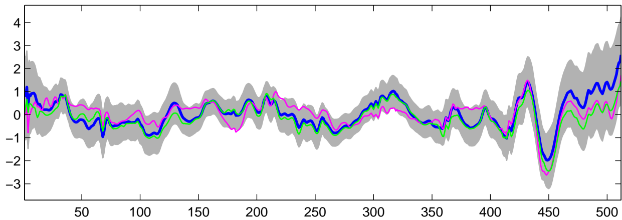
Estimated U_4(t) using G-WFMM: t_2 data, run 8
