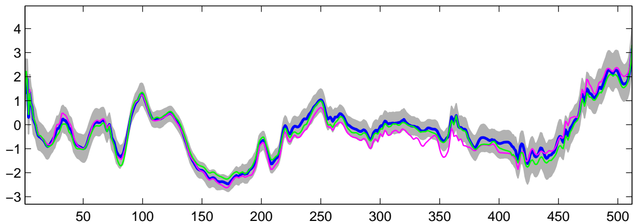
Estimated U_4(t) using R-WFMM: t_3 data, run 8
