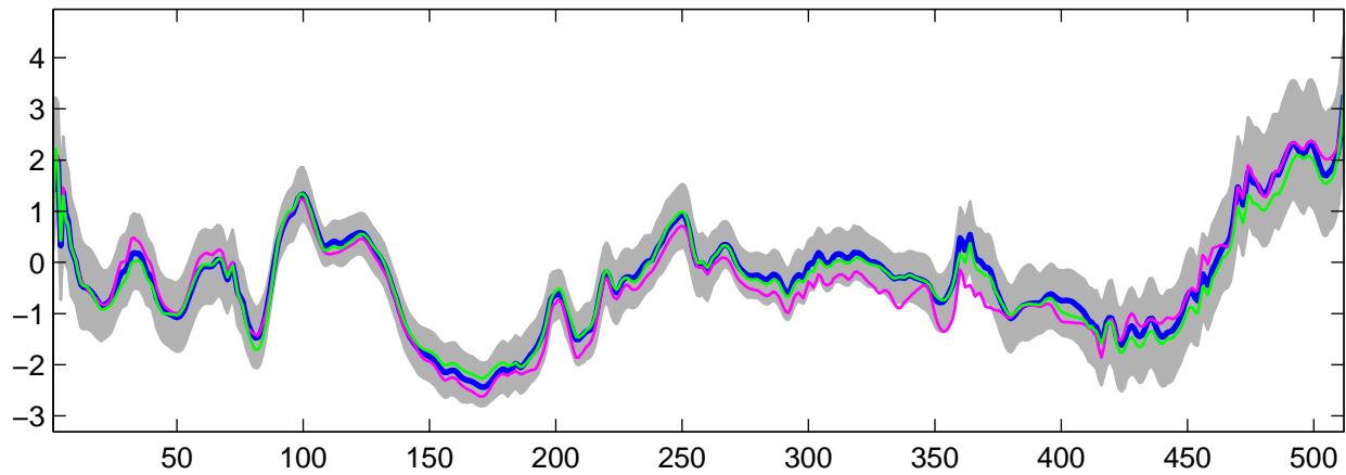
Estimated U_4(t) using G-WFMM: t_3 data, run 8
