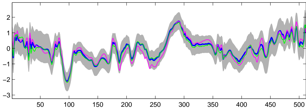
Estimated U_5(t) using G-WFMM: DE data, run 8
