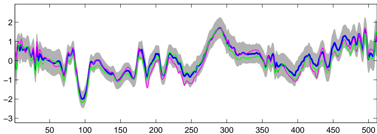
Estimated U_5(t) using R-WFMM: DE data, run 8
