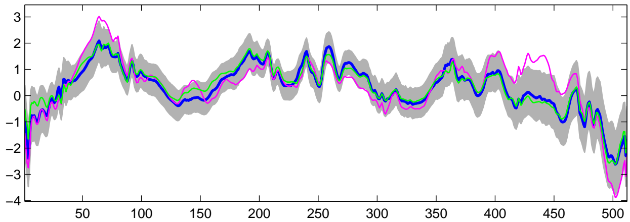
Estimated U_5(t) using R-WFMM: Normal data, run 8
