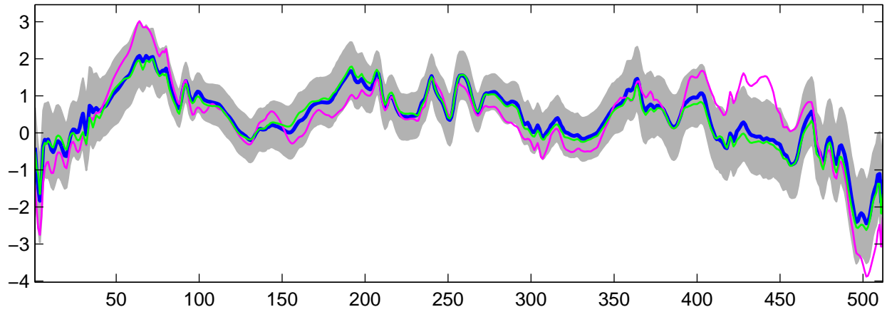
Estimated U_5(t) using G-WFMM: Normal data, run 8
