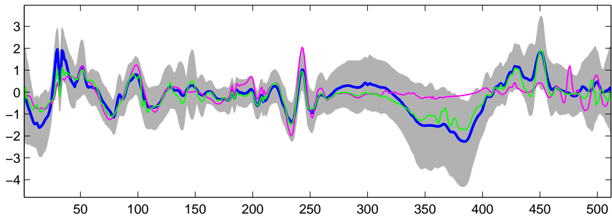
Estimated U_5(t) using G-WFMM: t_1 data, run 8
