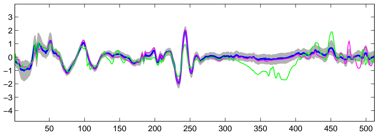
Estimated U_5(t) using R-WFMM: t_1 data, run 8
