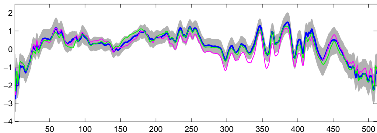
Estimated U_5(t) using R-WFMM: t_3 data, run 8
