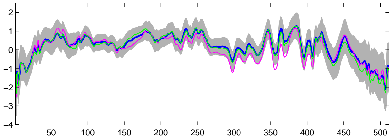
Estimated U_5(t) using G-WFMM: t_3 data, run 8
