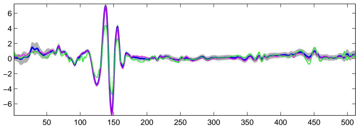
Estimated U_6(t) using R-WFMM: t_1 data, run 8
