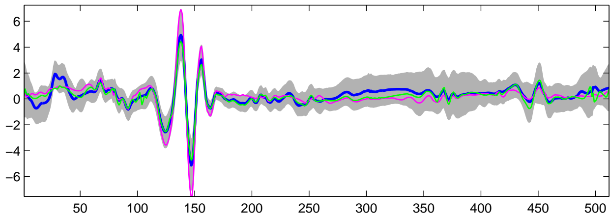
Estimated U_6(t) using G-WFMM: t_1 data, run 8
