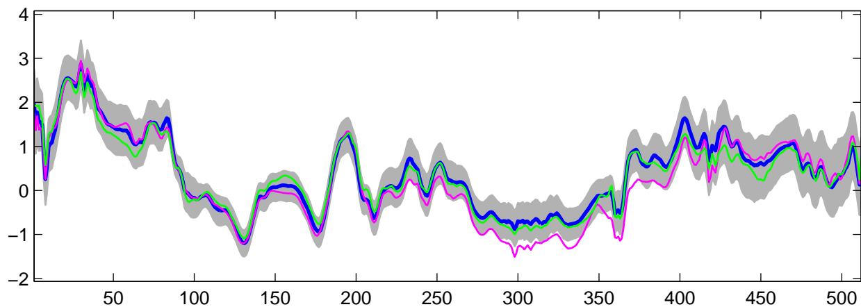
Estimated U_6(t) using R-WFMM: t_3 data, run 8
