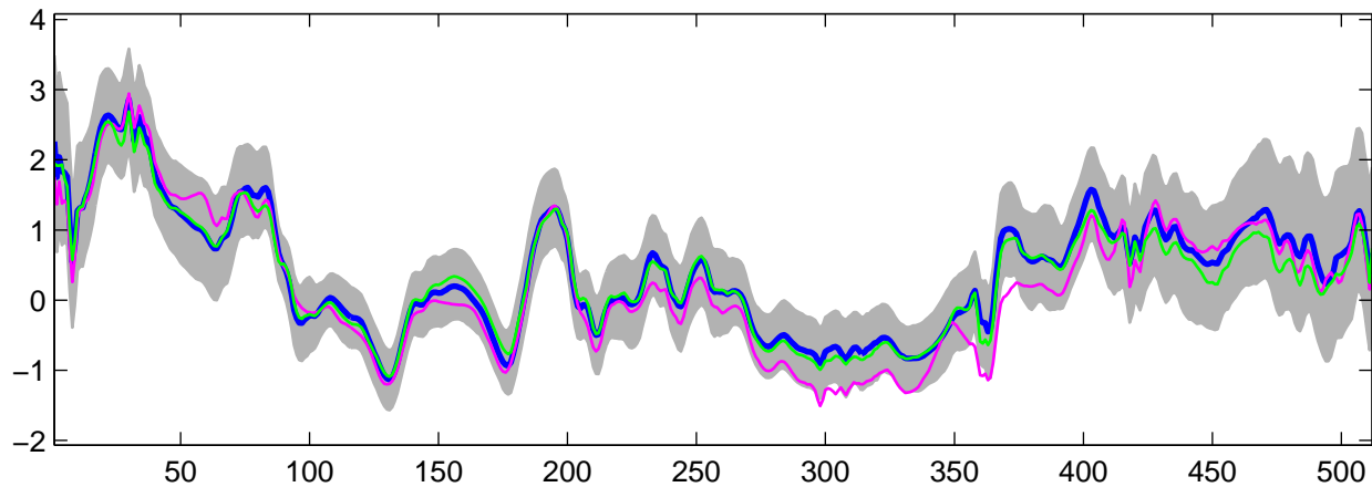
Estimated U_6(t) using G-WFMM: t_3 data, run 8
