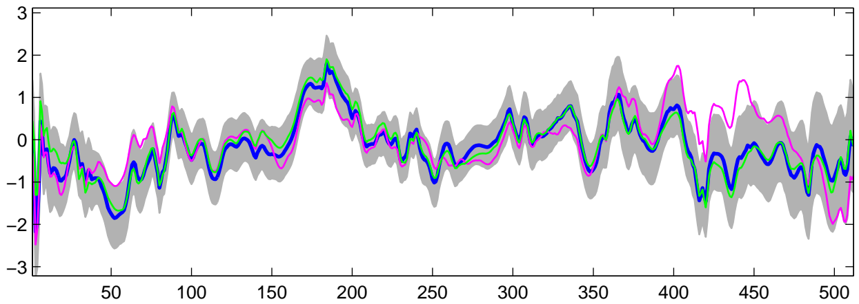
Estimated U_7(t) using R-WFMM: Normal data, run 8
