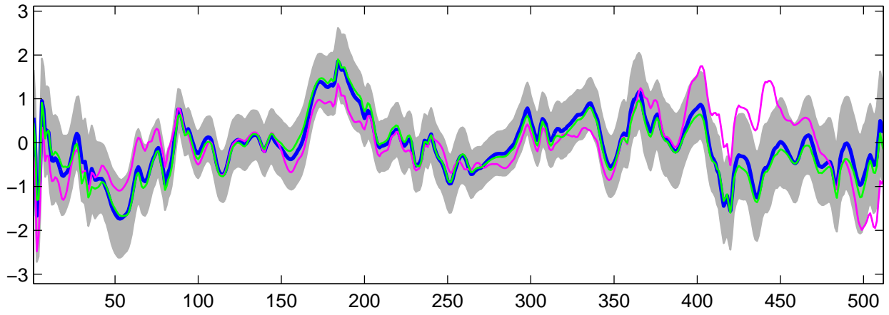
Estimated U_7(t) using G-WFMM: Normal data, run 8
