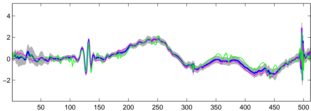
Estimated U_7(t) using R-WFMM: t_1 data, run 8
