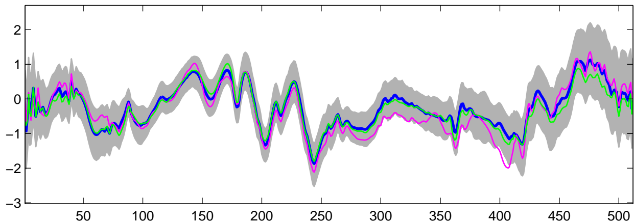
Estimated U_7(t) using G-WFMM: t_3 data, run 8
