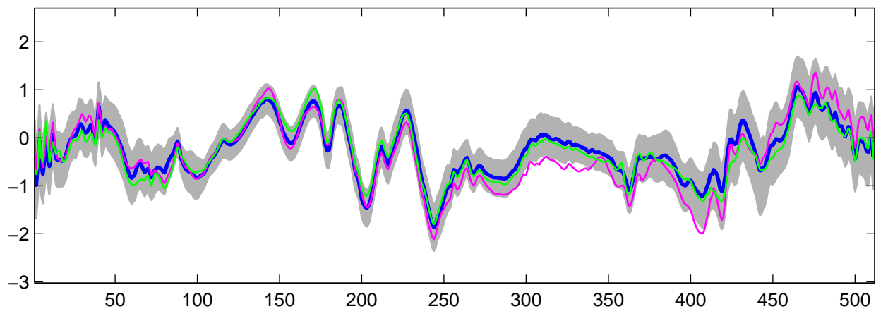
Estimated U_7(t) using R-WFMM: t_3 data, run 8
